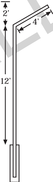
BACKSTOP W/OVERHANG SIDE VIEW
